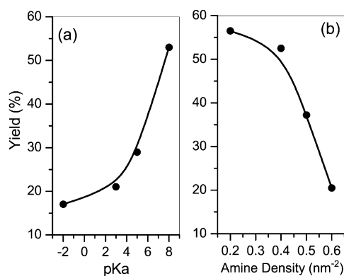
Figure 1. a) Effect of acid strength on the catalytic activity of the supported amine catalysts and b) effect of amine loading on the yield of dimer product. Reaction conditions: heptan-2-one (2 mmol, 0.228 g), Si–Al– \text{NHCH}_2\text{CH}_2\text{NH}_2 catalyst (0.1 g, 0.4 amines \text{nm}^{-2} ), t = 12 h, T = 443 K.
